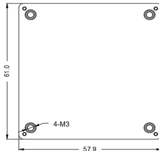
Standard 61.0X57.9X12.7mm
