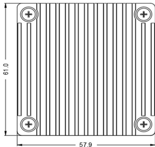
Standard+Heat sink 61.0X57.9X27.7mm
