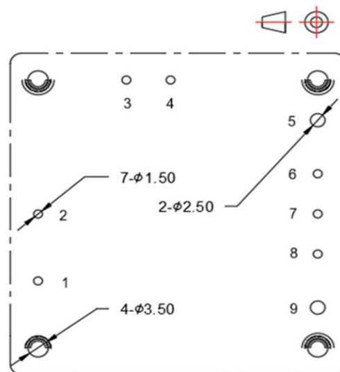
Recommended holes for PCB
